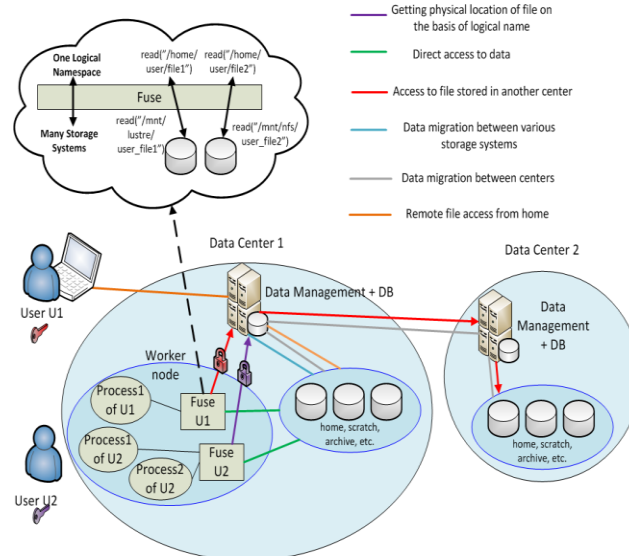
Fig:3- Proposed Architecture
